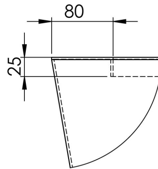
DETAIL E SCALE 1 : 5
