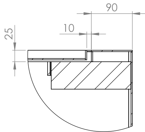
DETAIL K SCALE 1 : 5
