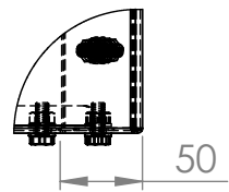
DETAIL B SCALE 1 : 5
