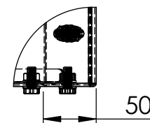
DETAIL B SCALE 1 : 5
